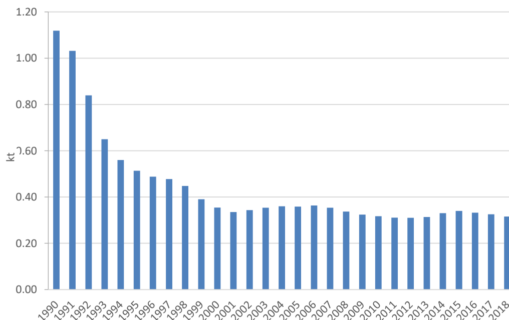
Figure 5-7. Direct N 2 O emission from manure management
