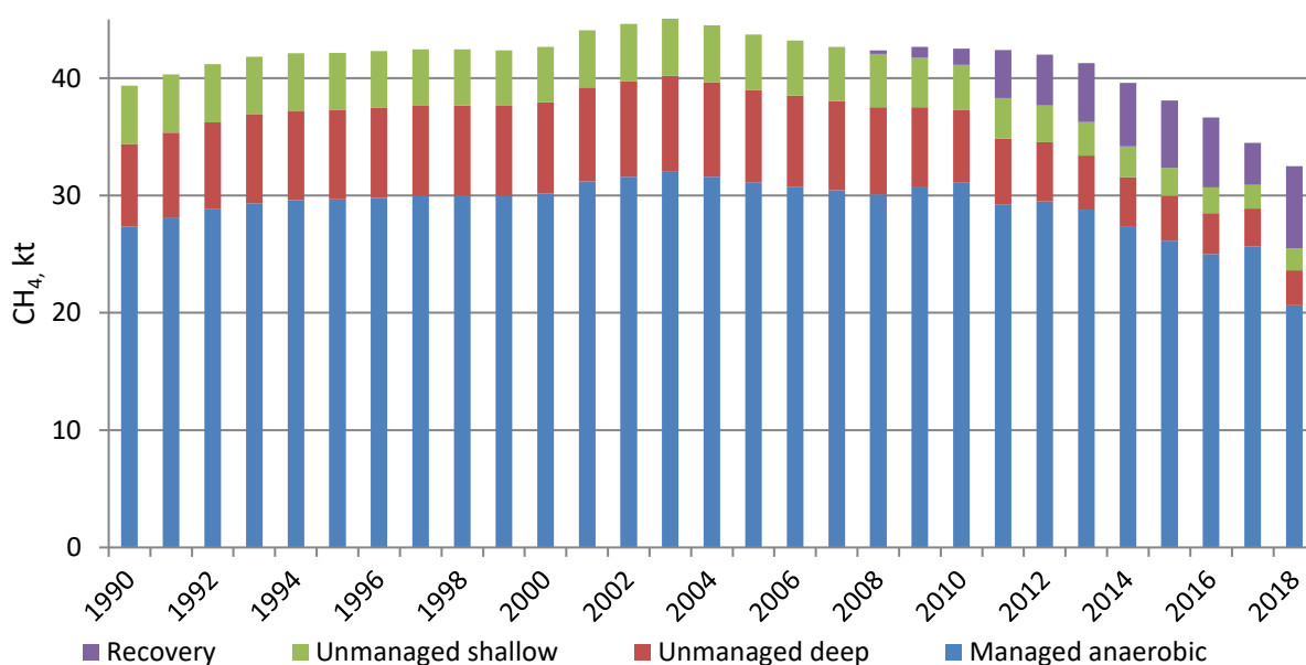
Figure 7-1. Variations of GHG emissions from solid waste disposal (1990-2018)
