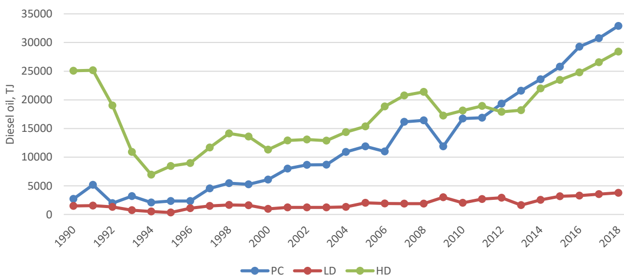
Figure 3-41. Diesel oil consumption per vehicle type for road transport 1990-2018
