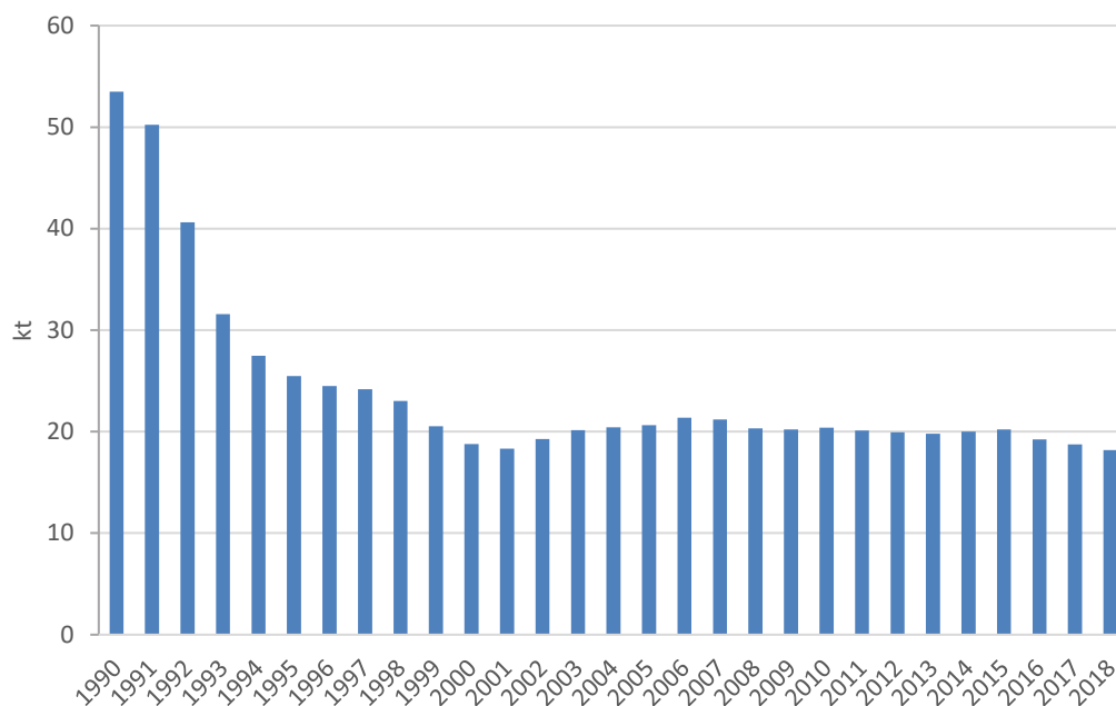
Figure 5-9. N losses due to volatilization of \text{NH}_3 and \text{NO}_x and leaching during the period 1990-2018
