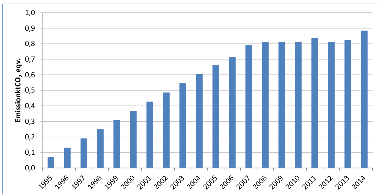
Figure 4-26. Fluorinated gas emissions from commercial refrigeration in accommodation and catering businesses for 1995-2014
