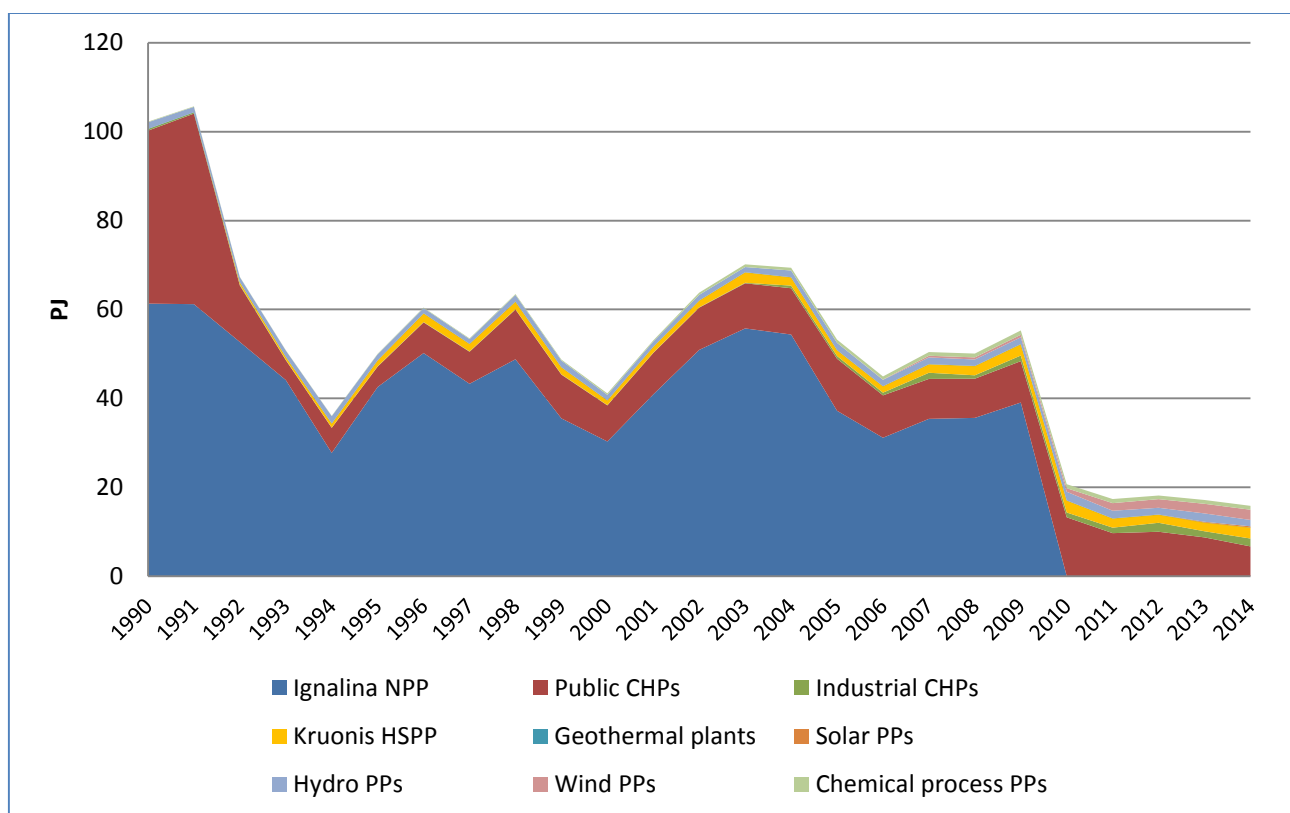
Figure 3-5. Structure of electricity generation in Lithuania
