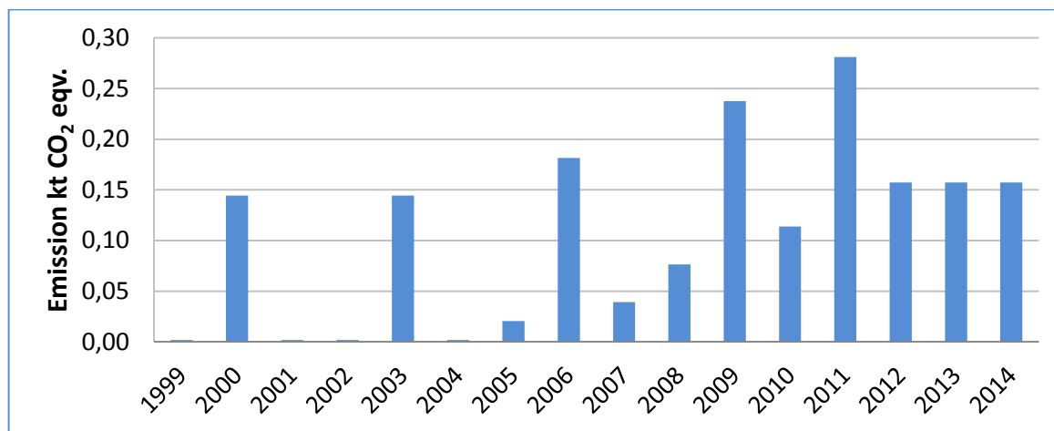
Figure 4-42. SF 6 emissions from accelerators (in radiation therapy facilities) for 1999-2014
