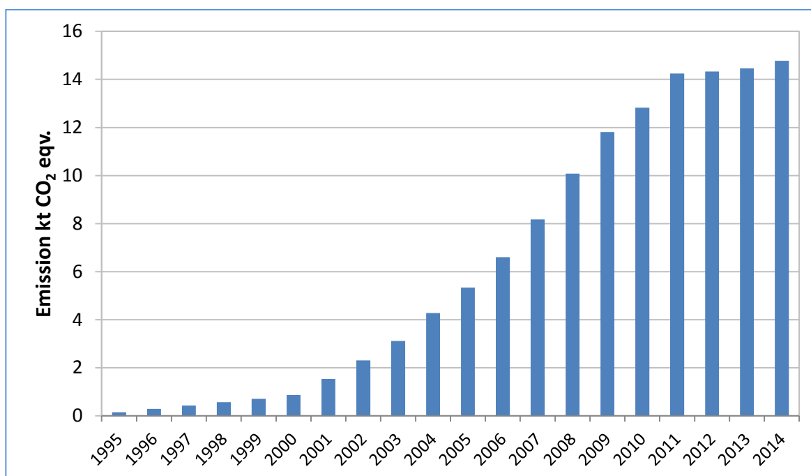
Figure 4-36. Fluorinated gas emissions from stationary air conditioning for 1995-2014
