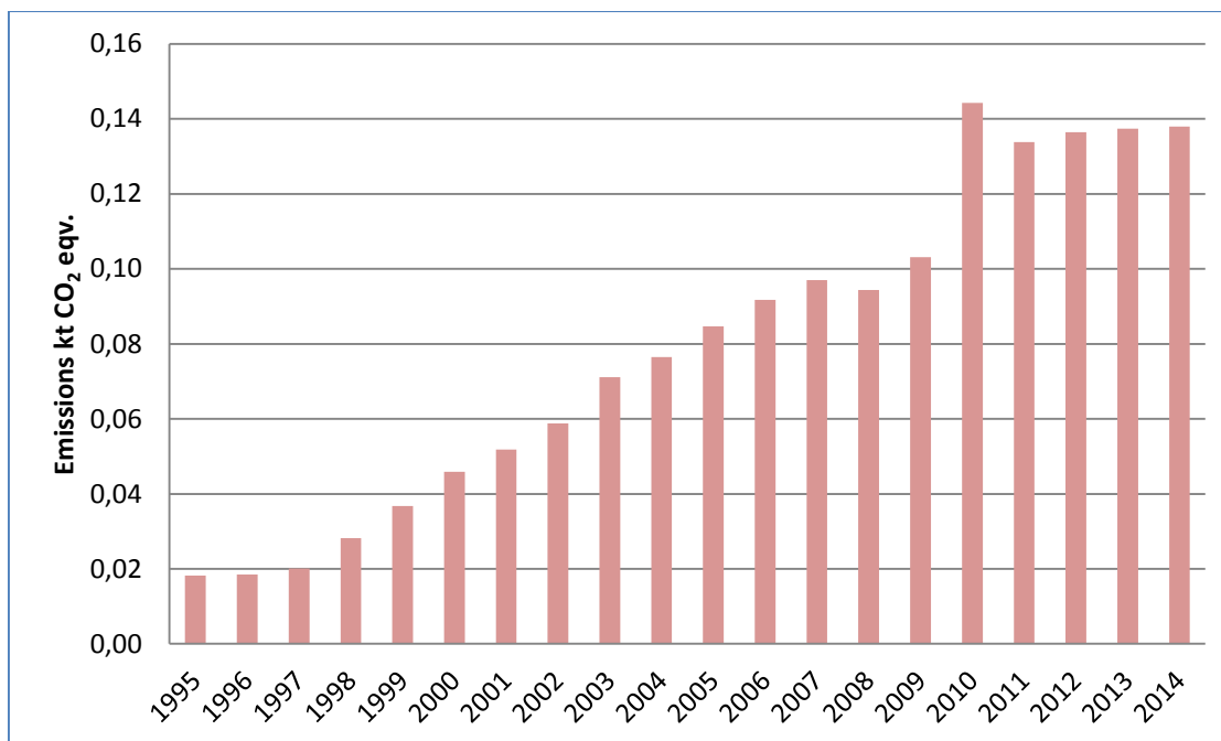
Figure 4-29. Fluorinated gas emissions from domestic freezers in Lithuania for 1995-2014
